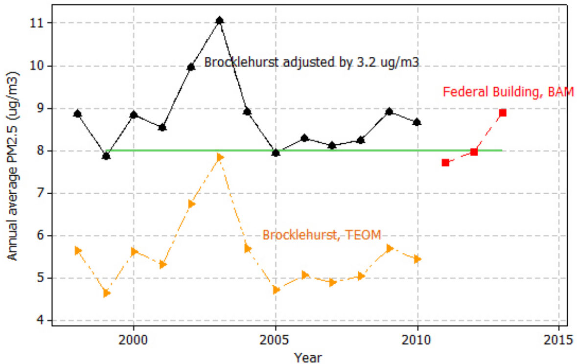
Figure 2: Annual average PM_{2.5} values for Kamloops. The black line shows the measured TEOM values adjusted by the offset factor calculated in this report. The green line is the BC MOE provincial guideline value of 8 \mu\text{g}/\text{m}^3 .
