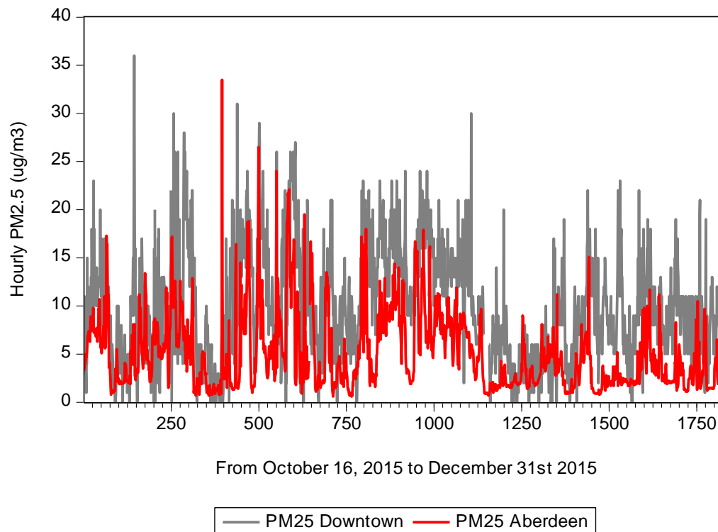
Figure 4: Hourly pattern of PM 2.5 concentrations at the Aberdeen and Federal Building (downtown) monitoring stations for the period noted.
