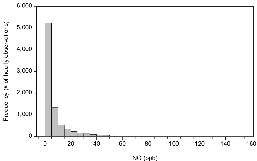
Figure 4: Distribution of hourly nitrogen oxide values for the downtown Kamloops monitoring station in 2015
