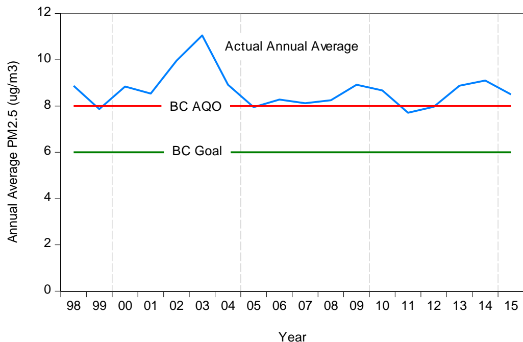
Figure 1: Historical Annual Average PM_{2.5} in Downtown Kamloops, 1998-2015. See Tsigaris and Schemenauer (2014b) for a discussion of the data analysis.
